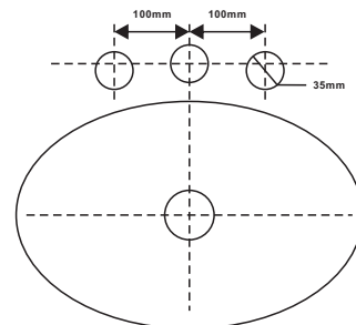
Faucet hole specification-2
